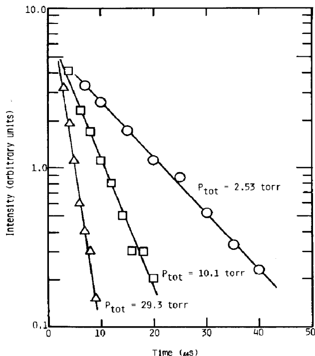
Fig. 5. Decay of the fast fluorescence component from 272 nm photolysis of \text{ClN}_3 - \text{Cl}_2 -Ar mixtures at several different total pressures ( X_{\text{ClN}_3} \approx 0.001 , X_{\text{Cl}_2} \approx 0.078 ).
