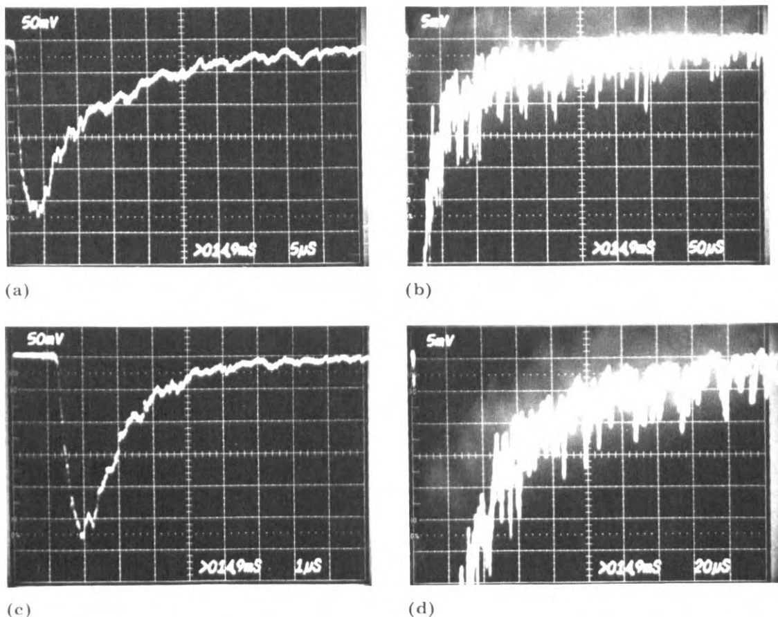
Fig. 4. \text{NCl}^* fluorescence following the photolysis of \text{ClN}_3\text{-Cl}_2\text{-Ar} mixtures at 272 nm ( X_{\text{ClN}_3} \approx 0.001 , X_{\text{Cl}_2} \approx 0.078 ): (a) pressure, 2.53 Torr; 50 mV = 40 photoelectrons \mu\text{s}^{-1} ; (b) pressure, 2.53 Torr, 5 mV = 4.0 photoelectrons \mu\text{s}^{-1} ; (c) pressure, 38.9 Torr; 50 mV = 503 photoelectrons \mu\text{s}^{-1} ; (d) pressure, 38.9 Torr; 5 mV = 4.0 photoelectrons \mu\text{s}^{-1} .
