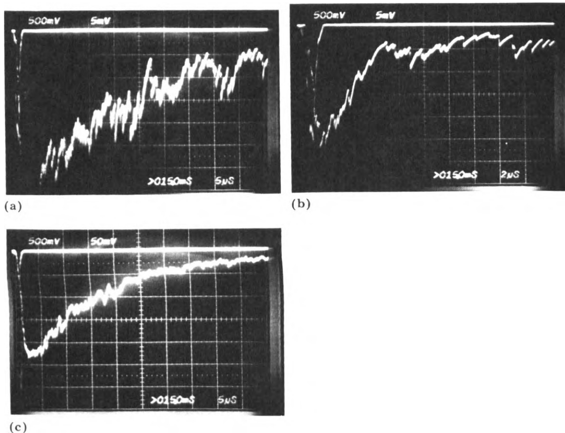
Fig. 1. \text{NCl}^* fluorescence following the photolysis of \text{ClN}_3\text{-Cl}_2\text{-Ar} mixtures at 300 nm ( X_{\text{ClN}_3} \leq 0.003 , X_{\text{Cl}_2} \approx 0.018 ): (a) shot 1, P_{\text{total}} = 1.1 Torr, 5 \text{ mV} = 4.0 photoelectrons \mu\text{s}^{-1} ; (b) shot 2, P_{\text{total}} = 1.1 Torr, 5 \text{ mV} = 4.0 photoelectrons \mu\text{s}^{-1} ; (c) shot 1, P_{\text{total}} = 5.2 Torr, 50 \text{ mV} = 43.1 photoelectrons \text{s}^{-1} .
