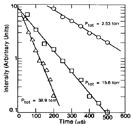
Fig. 5. Decay of the fast fluorescence component from 272 nm photolysis of \text{ClN}_3 - \text{Cl}_2 -Ar mixtures at several different total pressures ( X_{\text{ClN}_3} \approx 0.001 , X_{\text{Cl}_2} \approx 0.078 ).
