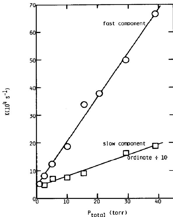
Fig. 7. Decay rates of fast and slow fluorescence components from 272 nm photolysis of \text{ClN}_3\text{-Cl}_2\text{-Ar} mixtures as a function of the total pressure ( X_{\text{ClN}_3} \approx 0.001 , X_{\text{Cl}_2} \approx 0.078 ).
