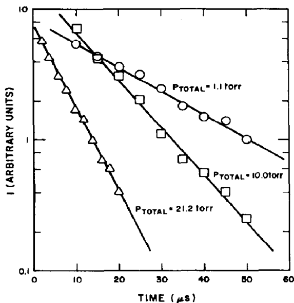
Fig. 2. \text{NCl}^* fluorescence decay at several different pressures following the photolysis of \text{ClN}_3\text{-Cl}_2\text{-Ar} mixtures at 300 nm ( X_{\text{ClN}_3} \lesssim 0.003 , X_{\text{Cl}_2} \approx 0.018 ).
