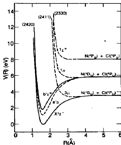
Fig. 8. Potential curves for ClN. Morse potentials with D_e values of 3.46 and 3.98 eV, r_e values of 1.61 and 1.56 Å and \omega_e values of 827 and 935.6 \text{cm}^{-1} are drawn for the X^3\Sigma^- and b^1\Sigma^+ states respectively. The estimated Morse parameters for the a^1\Delta state are D_e = 4.69 eV, r_e = 1.58 Å and \omega_e = 1000 \text{cm}^{-1} . The remaining three potential curves are Lennard-Jones potentials with C_6 = 2.21 \times 10^{-58} erg \text{cm}^6 as calculated from the Slater-Kirkwood formula using the method of Slater orbitals [51] to calculate the polarizability of nitrogen and chlorine, and with \sigma = 2.9 Å as calculated according to the rule of thumb given by Bernstein and Muckerman [52].
